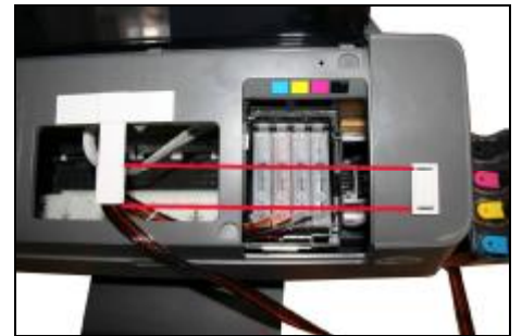
Stick the short support arm parallelly as the above picture shows.
